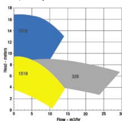
50 Hz, 1450 rpm
