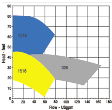
60 Hz, 1750 rpm
