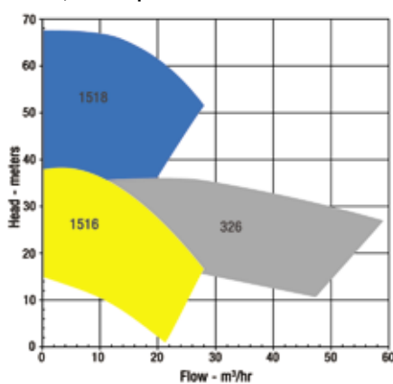
50 Hz, 1450 rpm
